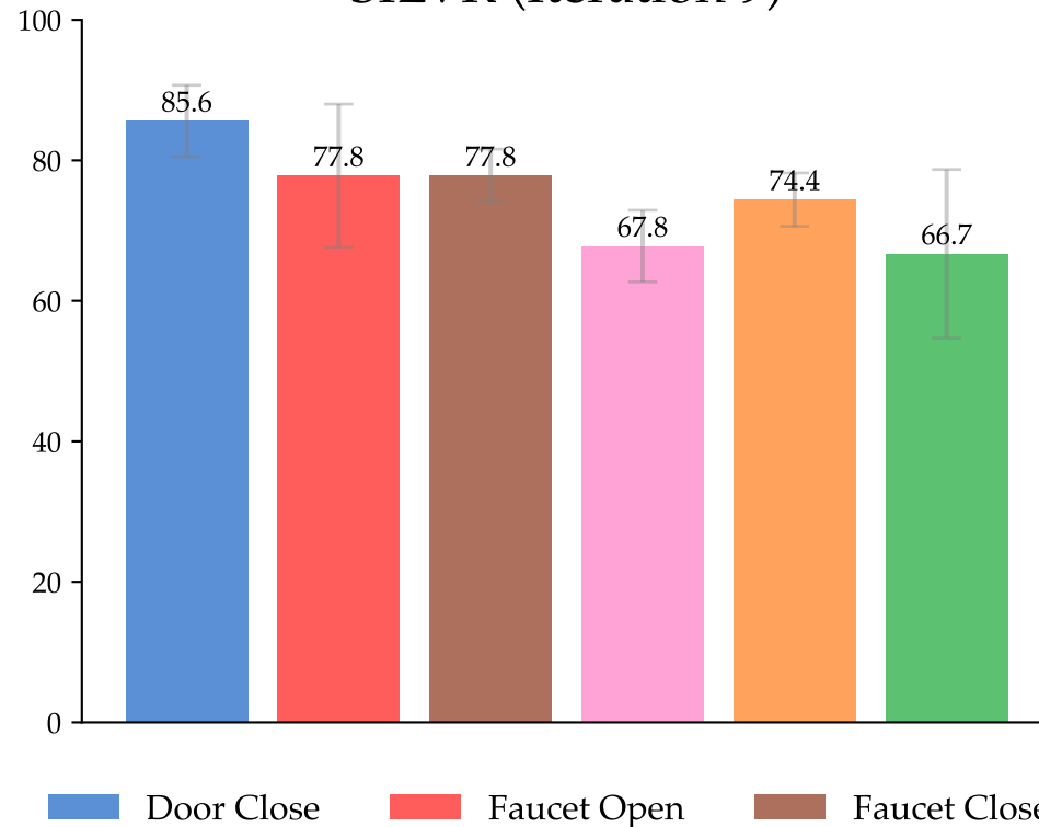
SILVR (Iteration 9)
