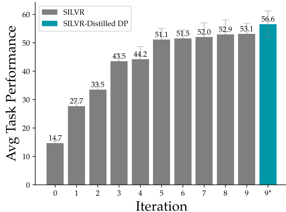
MetaWorld (10 Iterations)
