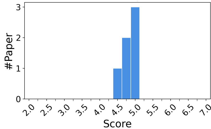
(b) GL-MCM
