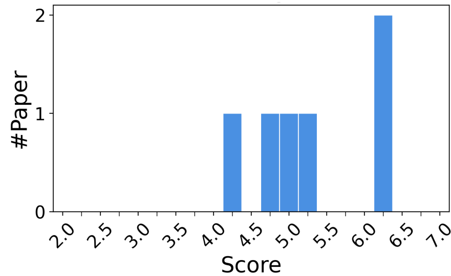
(c) Min-K%++
