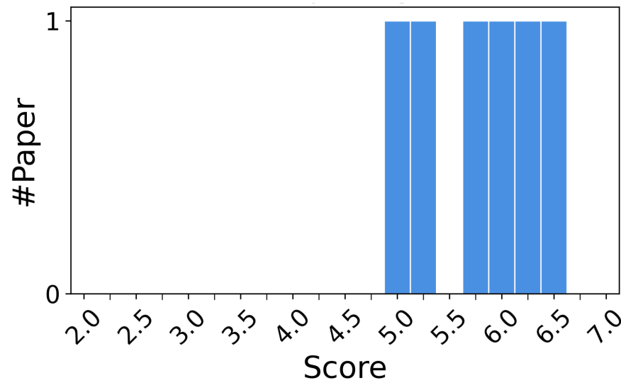
(a) LoCoOp
