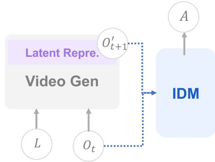
2(a) Latent Representation
