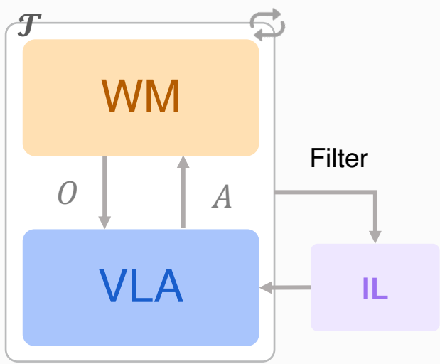
(a) Imitation Learning
