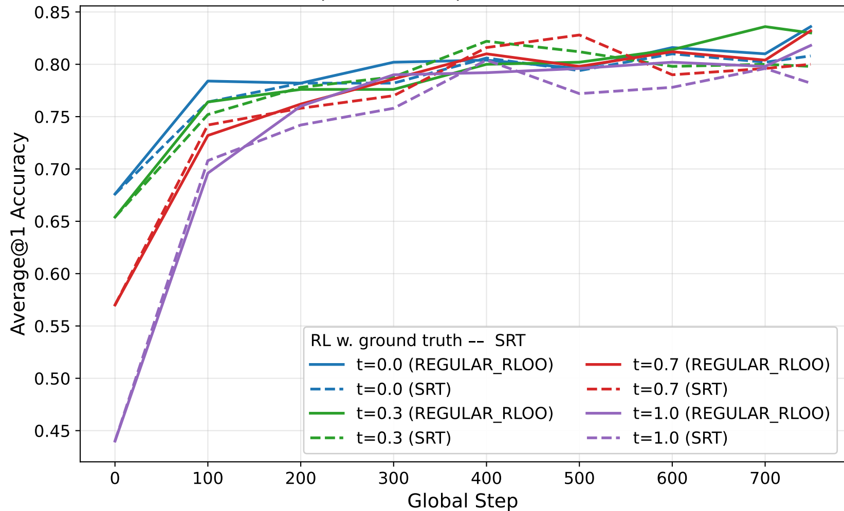
SRT vs Regular RL (Train: MATH) - Test: MATH
