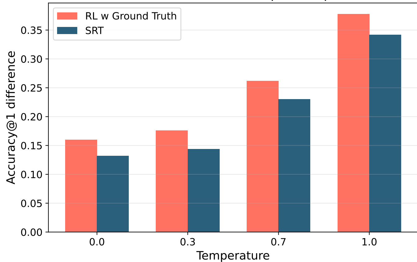
Absolute Performance Gain per Temperature
