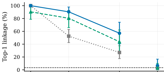
MOBIO / PolyProtect (N=30)
