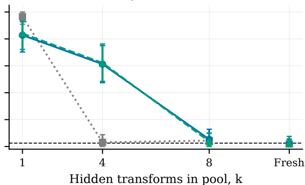
FEI / PolyProtect (N=40)
