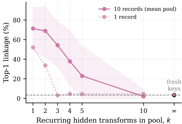
(b) MLP-Hash on MOBIO (chance 3.33%)
