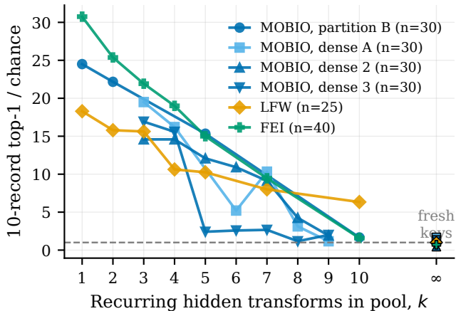
(a) BioHash, three datasets, chance-normalized
