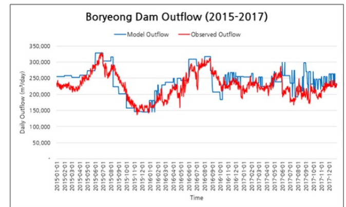
Fig. 5. Boryeong Dam outflow comparison: simulated vs. observed
