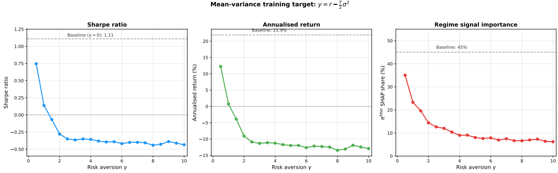
Figure 9: Performance and regime signal importance under mean-variance training targets with risk aversion \gamma \in [0.5, 10] . Left: Sharpe ratio drops from 1.11 at baseline to negative values by \gamma = 1.5 . Centre: annualised return declines from 21.9% to approximately -11\% . Right: \pi^{\text{filter}} SHAP share drops from 45% to below 10%, confirming that the variance penalty crowds out the regime signal. Dashed lines mark the baseline ( \gamma = 0 ).
