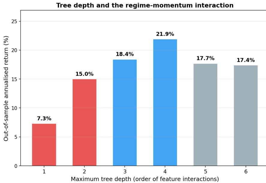
Figure 8: Out-of-sample annualised return as a function of maximum tree depth. Volatility is approximately constant ( \approx 19.5\% ) across all depths.
