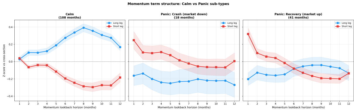
Figure 7: Momentum term structure by panic sub-type. Panic months are split by concurrent market return: crash (market down, 18 months) and recovery (market up, 41 months). The averaged panic profile in Figure 6 masks opposite selection patterns at months 7–12.
