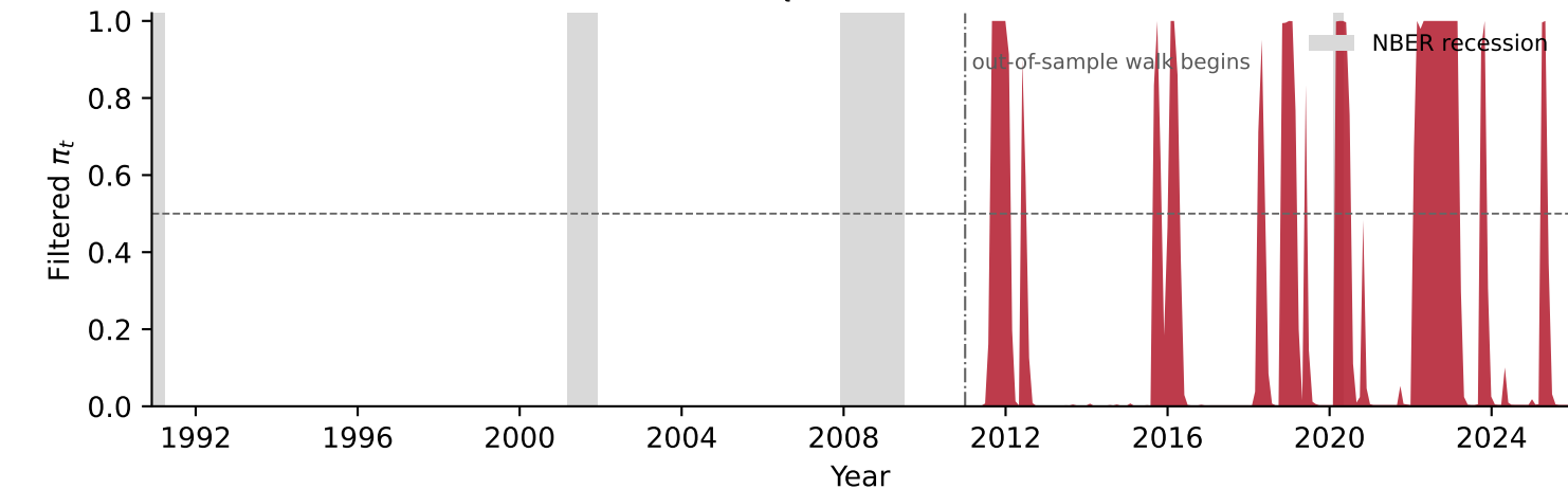
(b) Out-of-sample filtered panic probability \pi_t^{\text{filter}} (drawdown-only), 2011--2025
