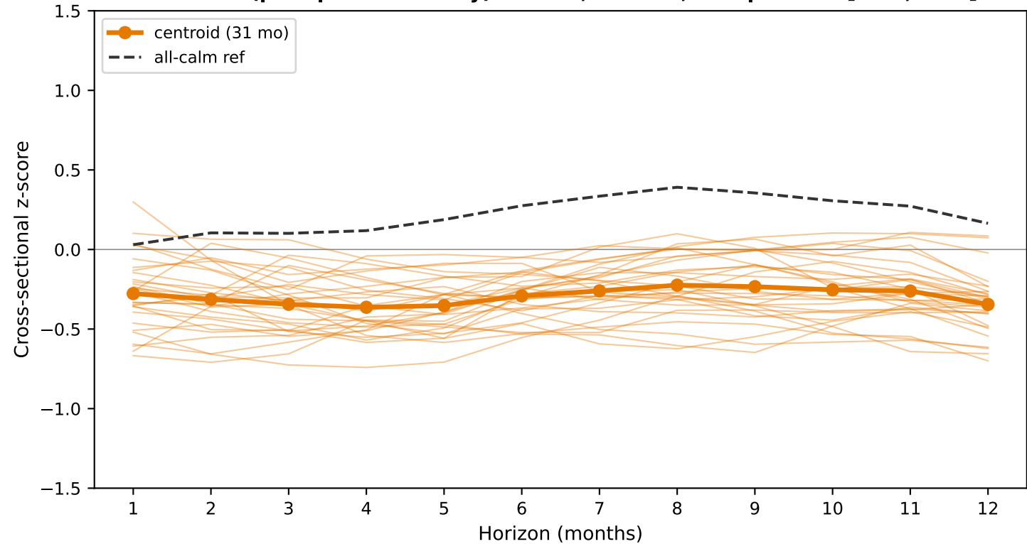
Cluster 2 (post-panic recovery) -- n=31 , \bar{\pi} = 0.32 , Sharpe=1.21 [0.18, 2.37]
