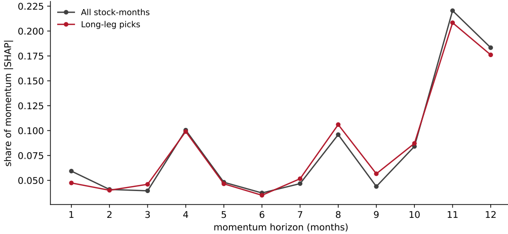
Figure 5: Per-horizon shares of momentum |\text{SHAP}| in the main model’s predictions, applied configuration: all out-of-sample stock-months versus the long-leg picks.
