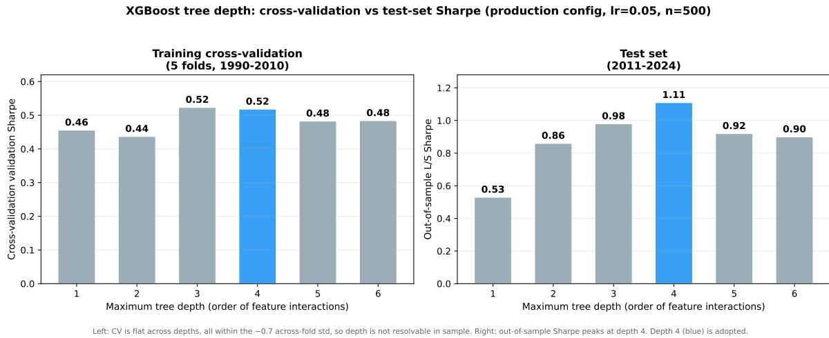
Figure 9: XGBoost tree-depth response at the production hyperparameters (learning rate 0.05, 500 trees). Left: five-fold expanding-window cross-validation validation Sharpe on the training period (1990–2010); the response is flat across depths, all within the across-fold standard deviation of roughly 0.7, so no depth is separable in sample. Right: out-of-sample long-short Sharpe on the 2011–2024 test window, which peaks at depth 4. Depth 4 (blue) is the adopted depth.
