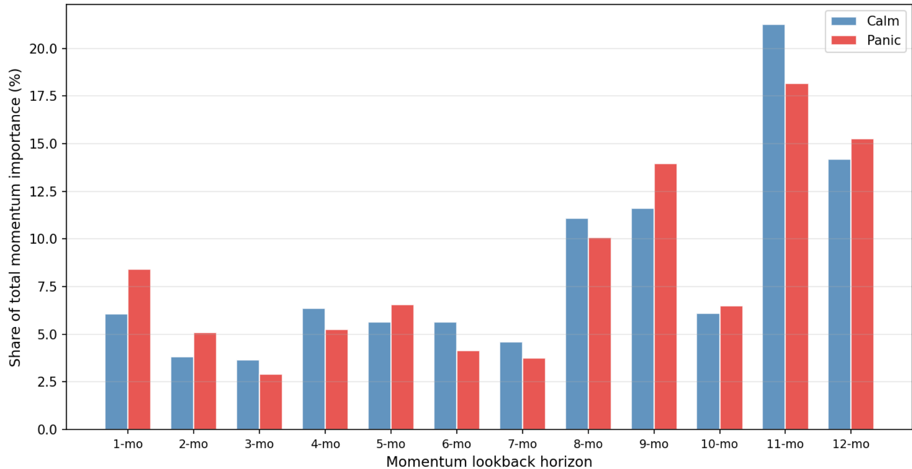
Distribution of model attention across momentum horizons: calm vs panic
