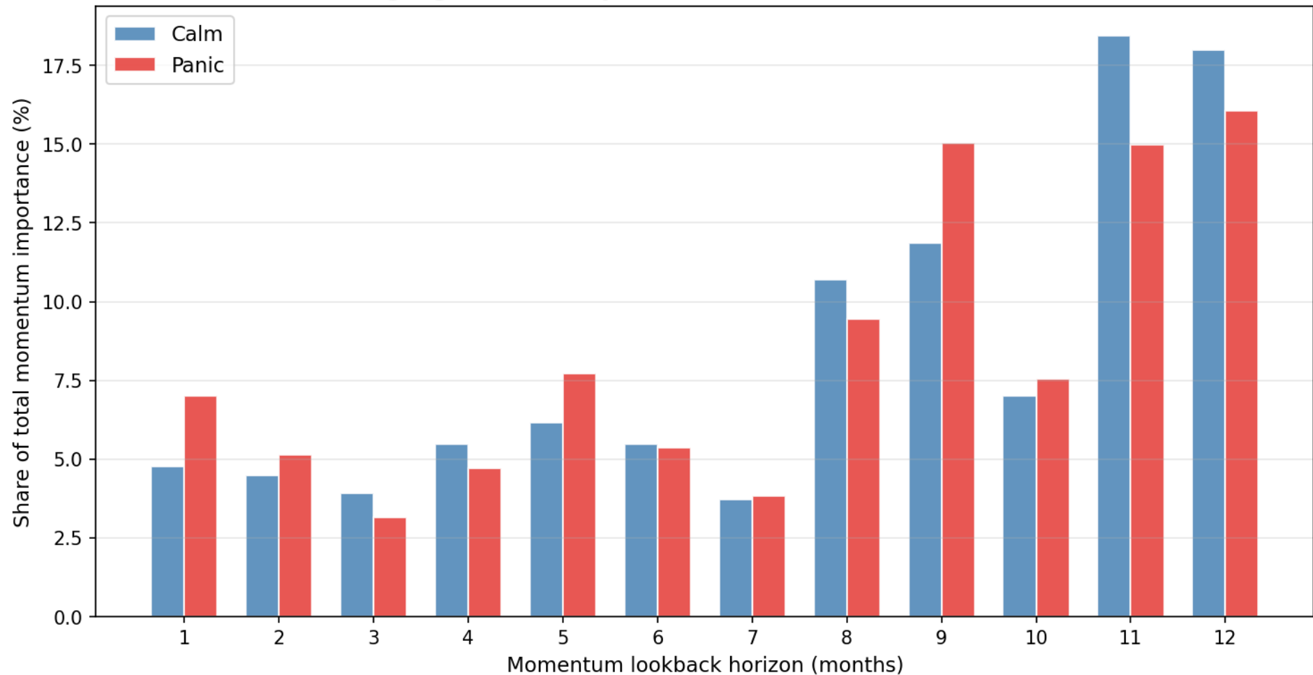
Long leg: relative importance of each momentum horizon
