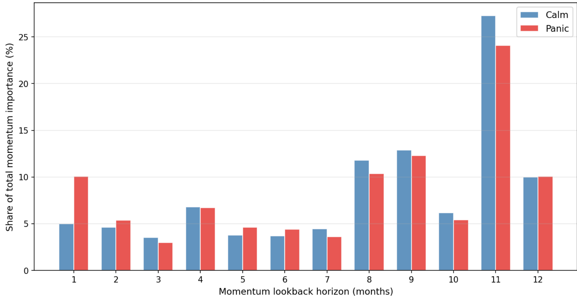
Short leg: relative importance of each momentum horizon
