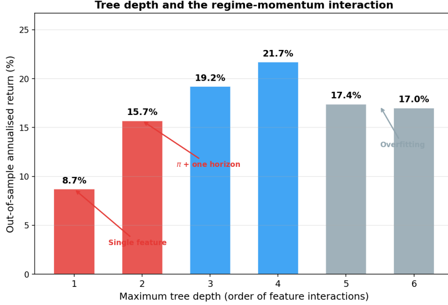
Figure 10: Out-of-sample annualised return as a function of maximum tree depth. Volatility is approximately constant ( \approx 19.5\% ) across all depths.
