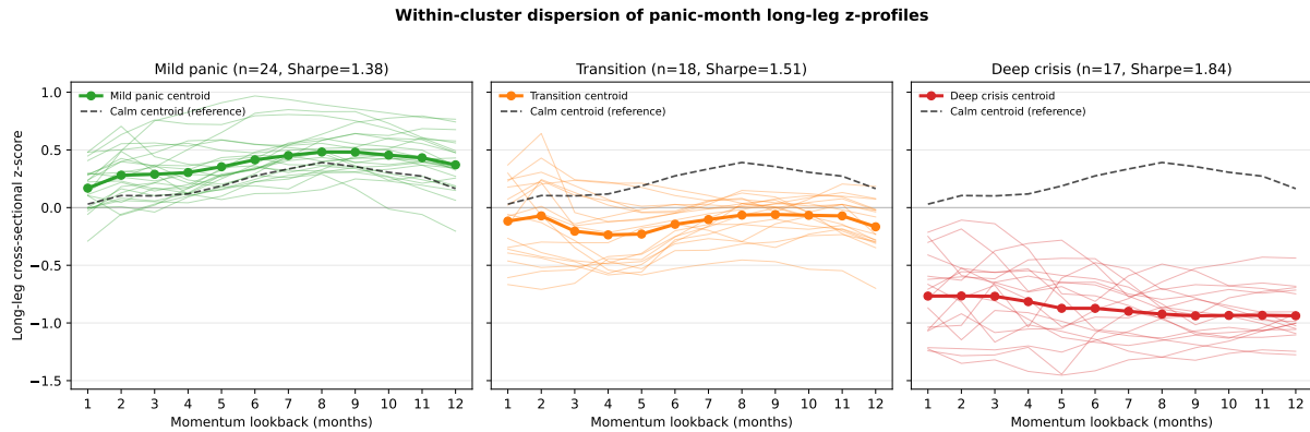
Figure 8: Within-cluster dispersion of panic-month long-leg z -profiles. Each panel plots all member-month profiles (thin lines) against the cluster centroid (heavy line); the dashed line is the calm centroid for reference. The mild-panic centroid is closer to the calm centroid (L2 distance 0.54) than the average mild-panic month is to its own cluster centroid (0.63).
