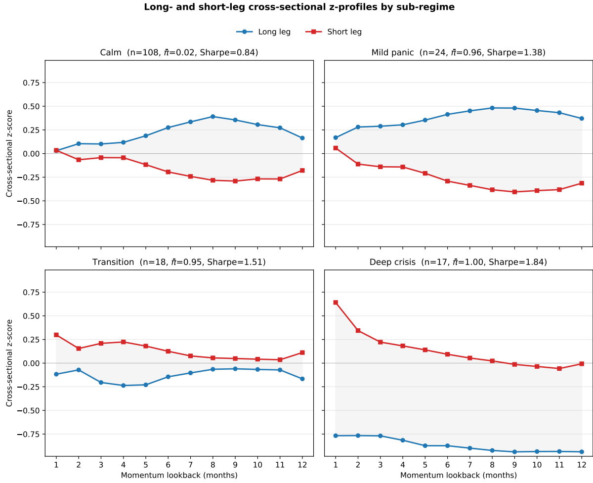
Figure 9: Long- and short-leg cross-sectional z-profiles by sub-regime. Mild panic (top right) is qualitatively similar to calm (top left) despite mean \pi^{\text{filter}} = 0.96 ; deep crisis (bottom right) shows the term-structure-wide loser pattern in pure form, with a short-leg z-spike of +0.64 at month 1.
