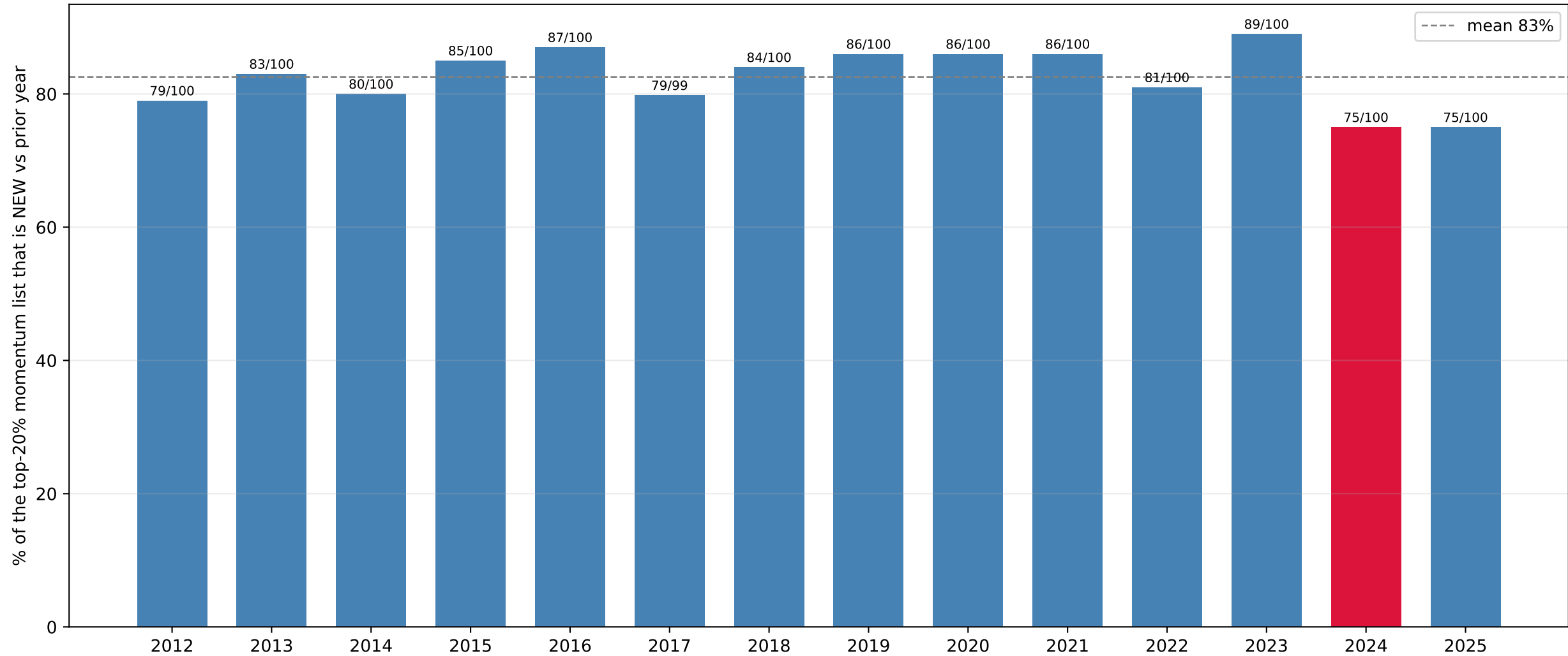
Year-over-year churn of SPMO's top-20% (top-quintile) momentum universe (labels = new names / list size; high = leadership rotated, low = winners persisted; red=2024)
