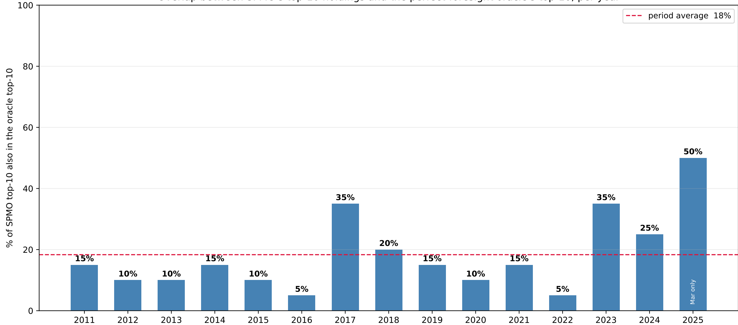
How often were SPMO's 10 biggest bets the RIGHT bets? Overlap between SPMO's top-10 holdings and the perfect-foresight oracle's top-10, per year
