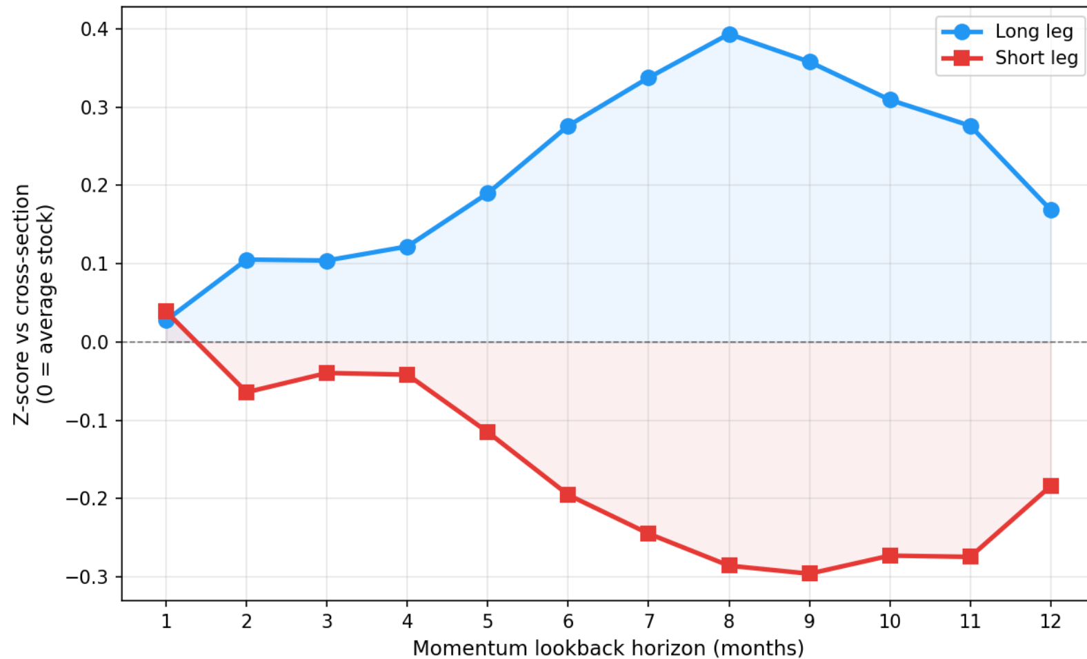
Calm: what stocks are selected (z-score of momentum vs cross-section)
