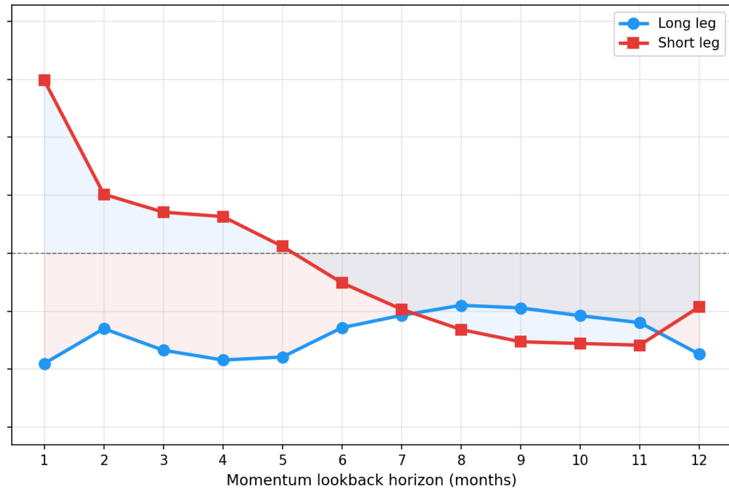
Panic: what stocks are selected (z-score of momentum vs cross-section)
