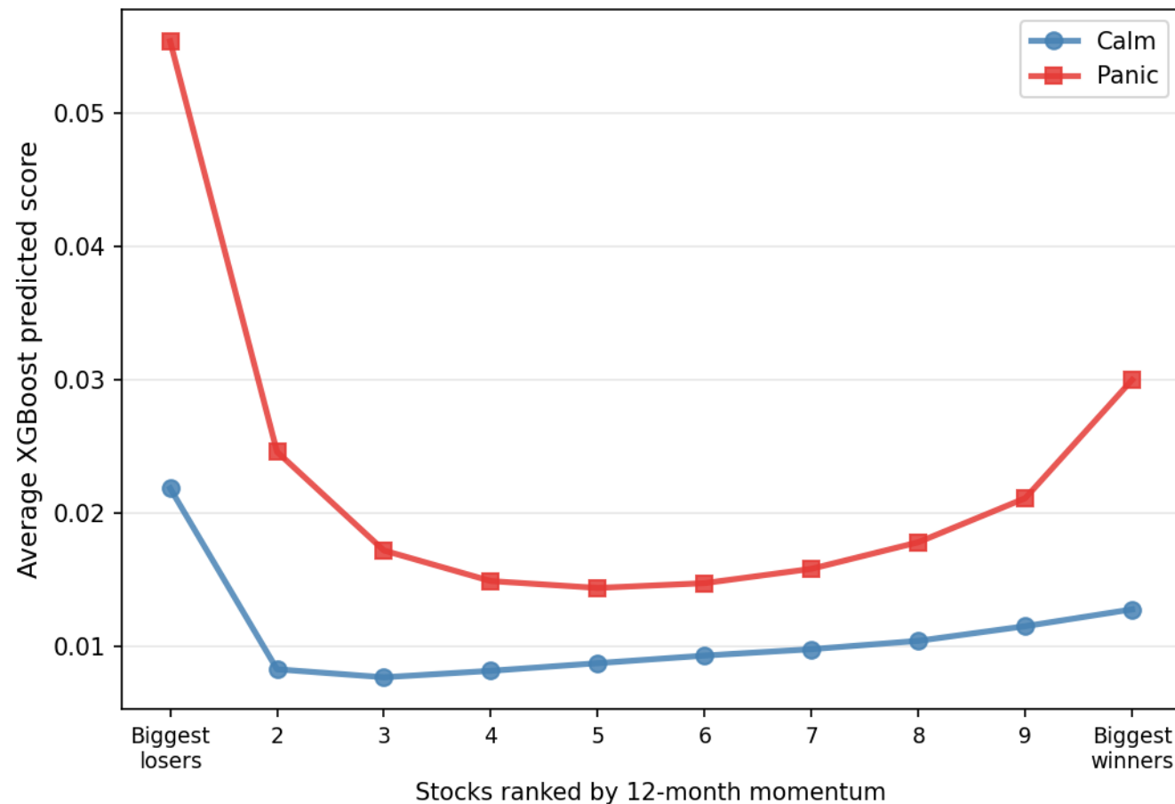
12-month momentum
