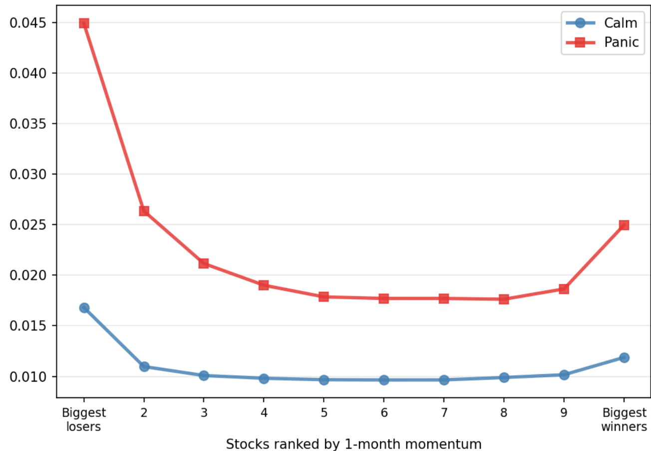
1-month momentum
