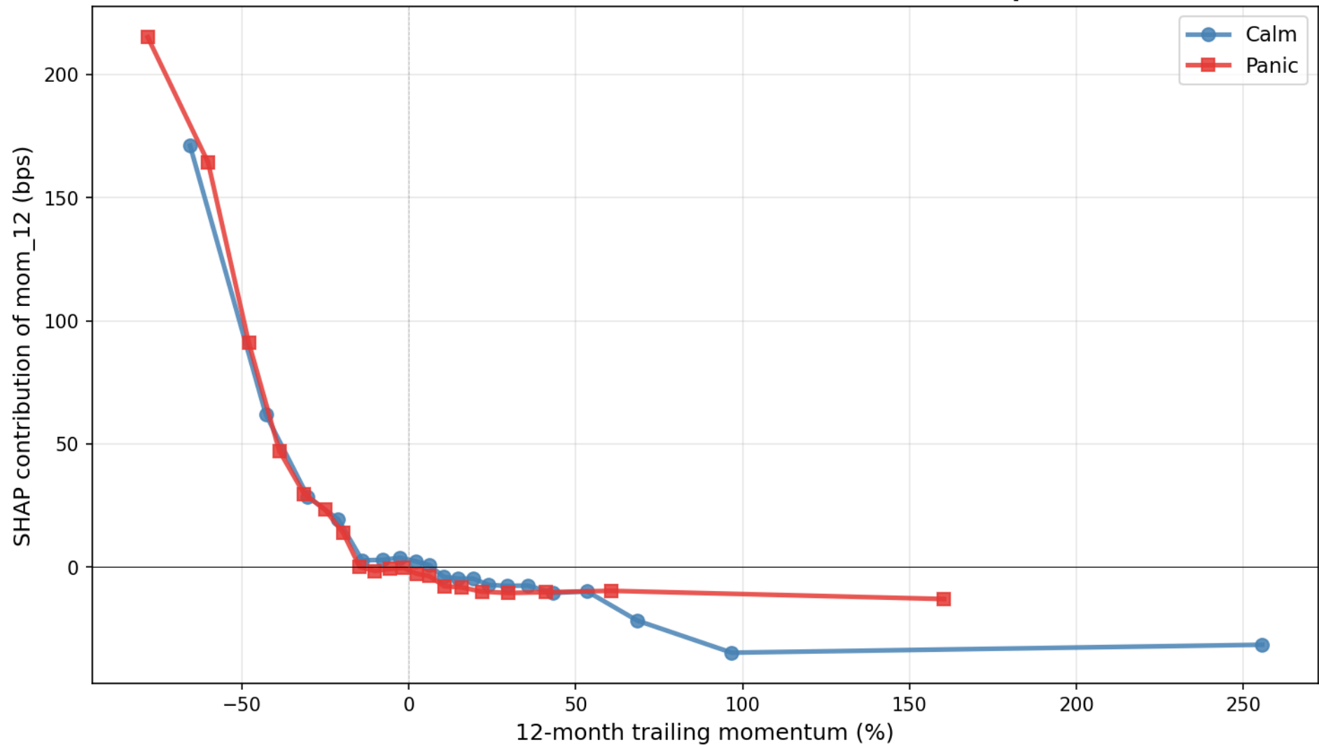
How XGBoost uses 12-month momentum: calm vs panic
