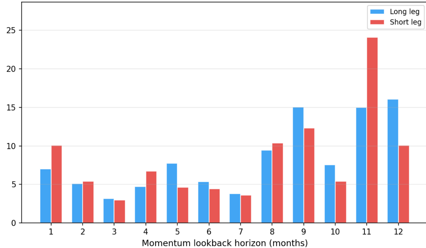
Panic: share of momentum importance by horizon (% of total |SHAP|, each group sums to 100%)
