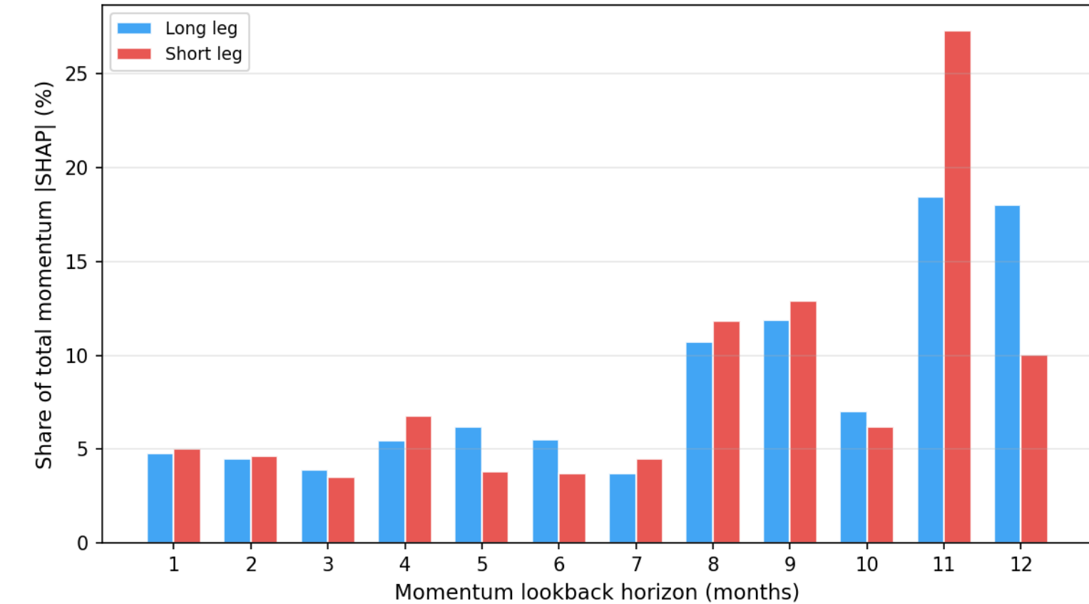
Calm: share of momentum importance by horizon (% of total |SHAP|, each group sums to 100%)
