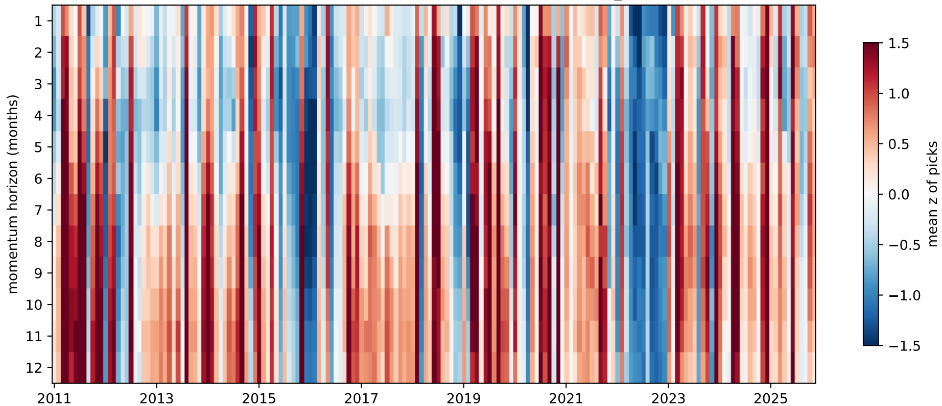
Applied long-leg picks: cross-sectional momentum z-curves by month (rule_r)
