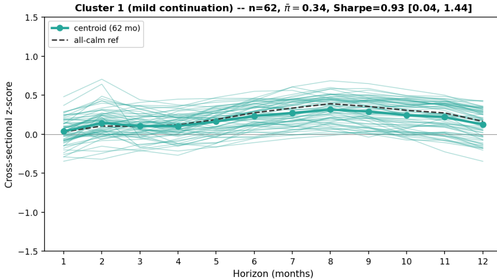
Figure 9: Cluster 1 (mild continuation): z-curves of the 62 member months, centroid, and all-calm reference.
