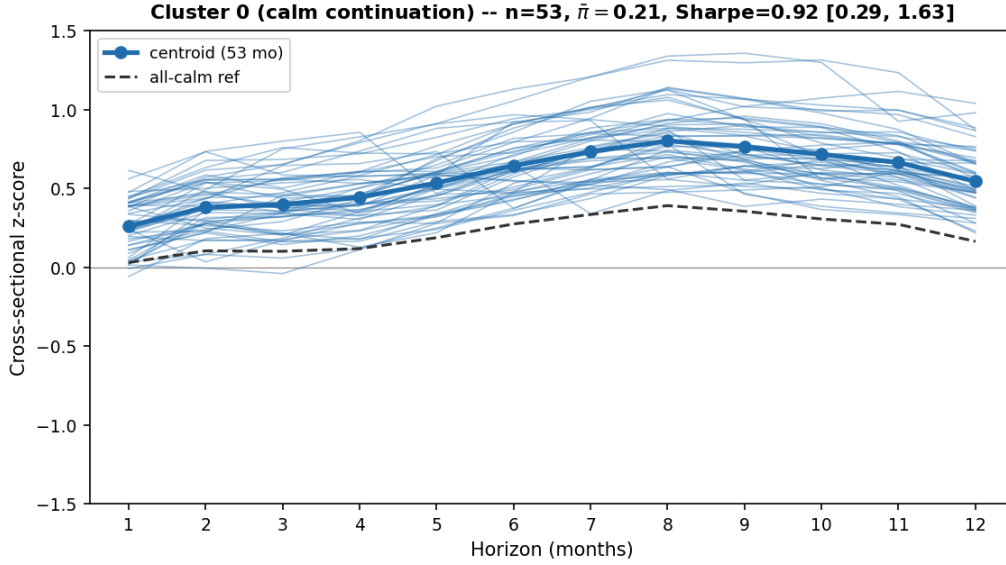
Figure 8: Cluster 0 (calm continuation): z-curves of the 53 member months, centroid, and all-calm reference.
