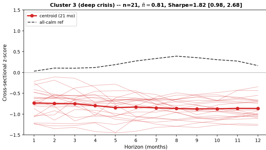
Figure 11: Cluster 3 (deep crisis): z-curves of the 21 member months, centroid, and all-calm reference.
