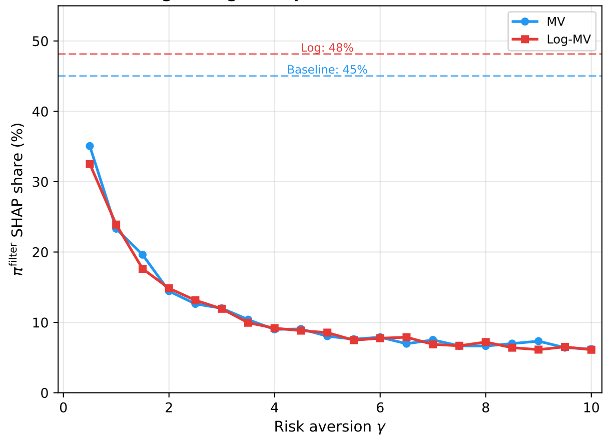
Regime signal importance vs risk aversion
