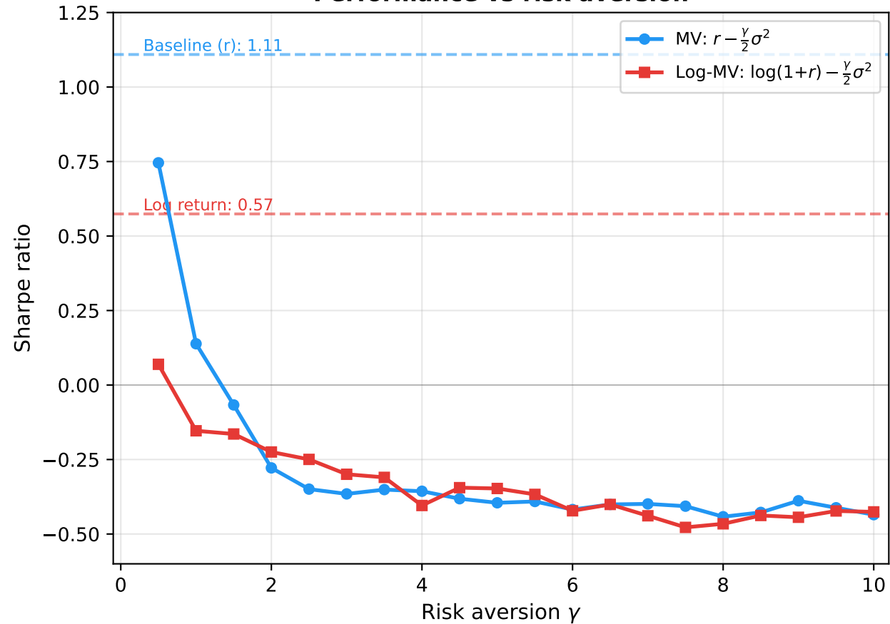
Performance vs risk aversion
