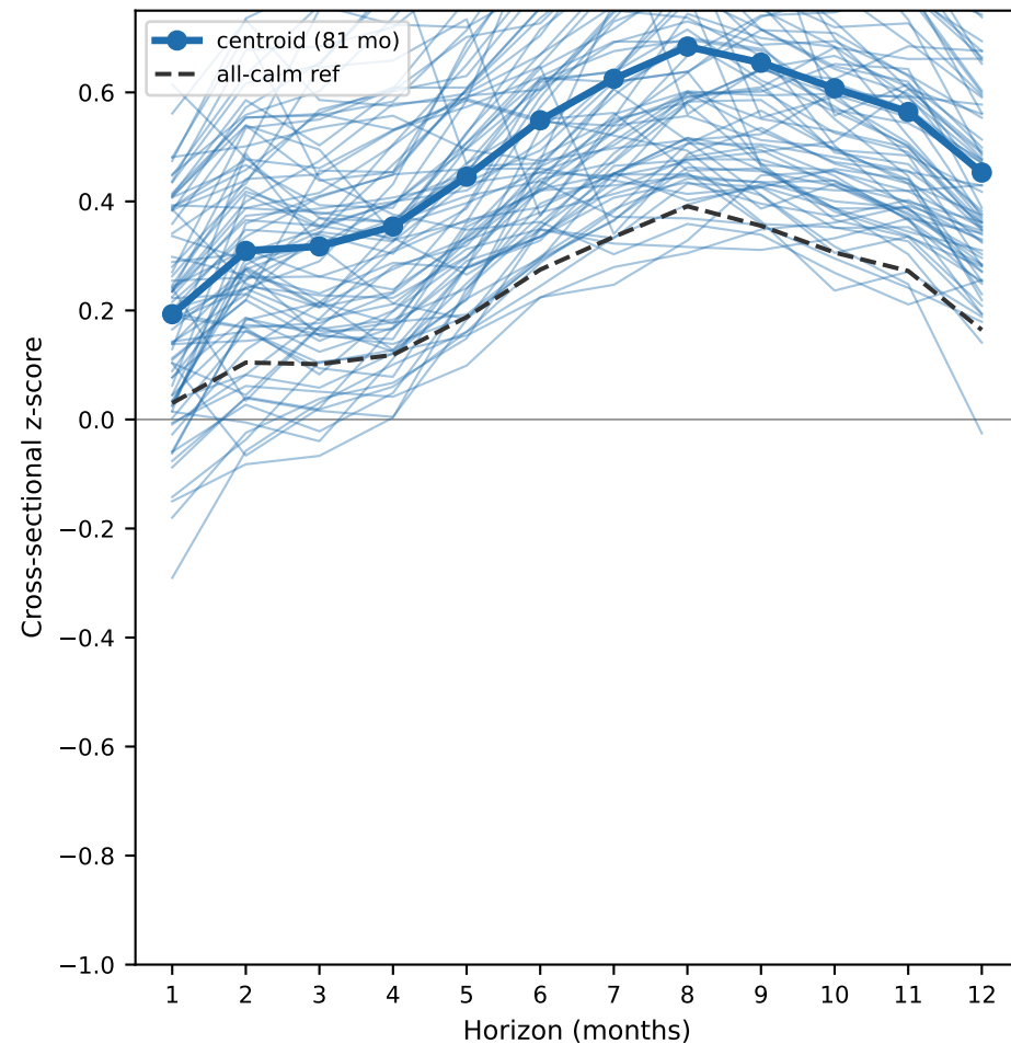
Cluster 0 ( n=81 , \bar{\pi}=0.26 ) Sharpe=0.85 [0.11, 1.52]
