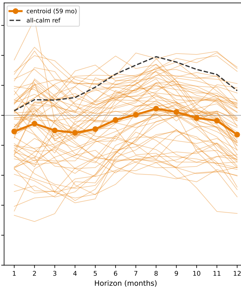
Cluster 1 ( n=59 , \bar{\pi}=0.34 ) Sharpe=1.34 [0.85, 1.91]
