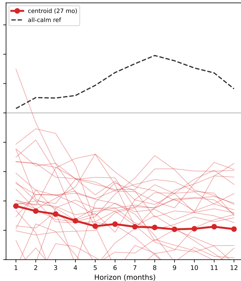
Cluster 2 ( n=27 , \bar{\pi}=0.67 ) Sharpe=1.23 [0.21, 1.78]
