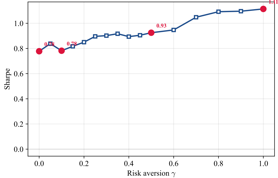
Sharpe Ratio
