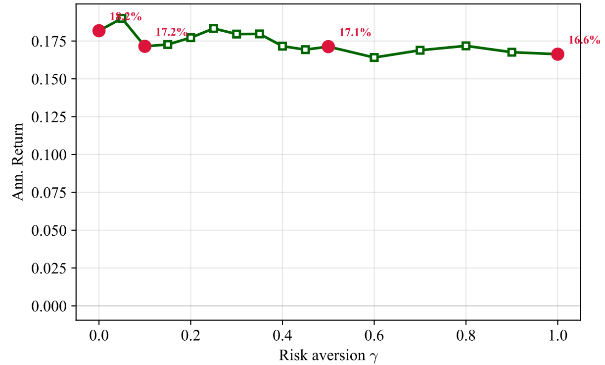
Annualised Return
