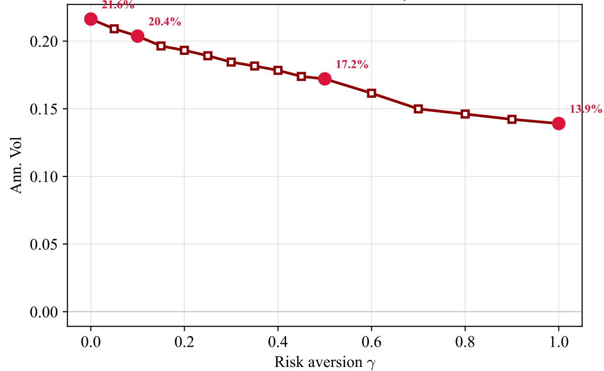
Annualised Volatility
