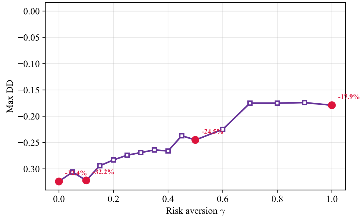
Maximum Drawdown
