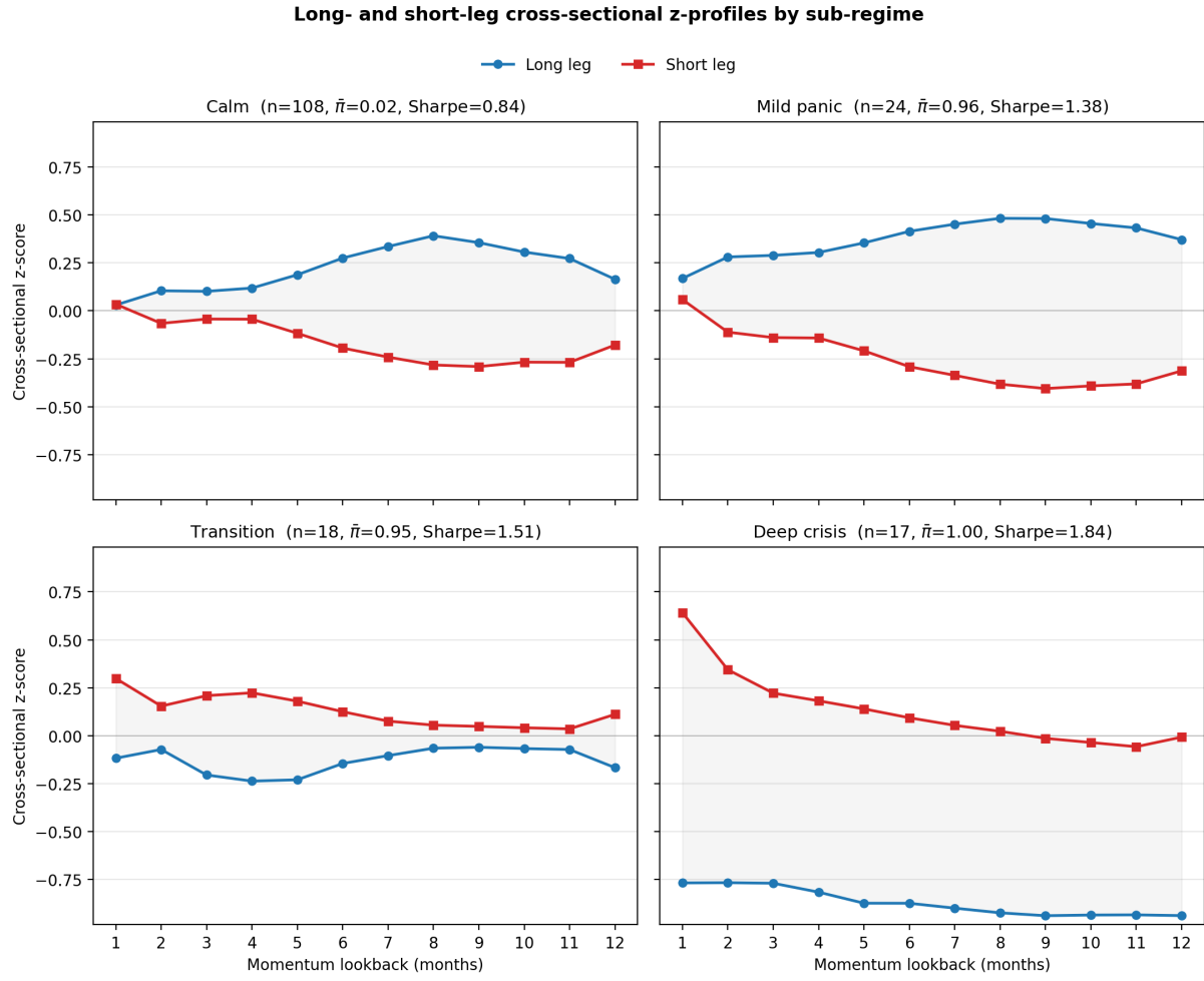
Figure 10: Long- and short-leg cross-sectional z -profiles by sub-regime. Calm is shown alongside the three panic sub-regimes obtained by K -means clustering of long-leg z -profiles ( k = 3 , random seed 42).
