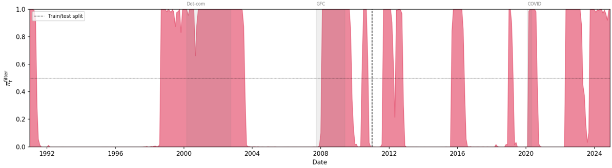
Figure 3: Filtered regime probability \pi_t^{\text{filter}} (1990–2025). The pink area shows the filtered probability path. The dashed vertical line marks the train/test split (January 2011), the dotted horizontal line marks the 0.5 threshold above which a month is classified as panic, and the grey vertical bands mark NBER recession periods. Major stress episodes (Dot-com, GFC, COVID) are labeled at the top.
