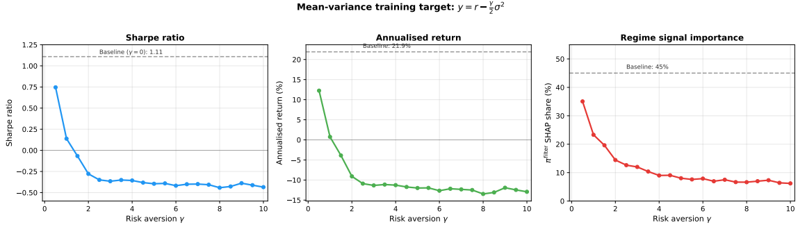
Figure 9: Performance and regime signal importance under mean-variance training targets with risk aversion \gamma \in [0.5, 10] . Left: Sharpe ratio drops from 1.11 at baseline to negative values by \gamma = 1.5 . Centre: annualised return declines from 21.9% to approximately -11\% . Right: \pi^{\text{filter}} SHAP share drops from 45% to below 10%, confirming that the variance penalty crowds out the regime signal. Dashed lines mark the baseline ( \gamma = 0 ).
