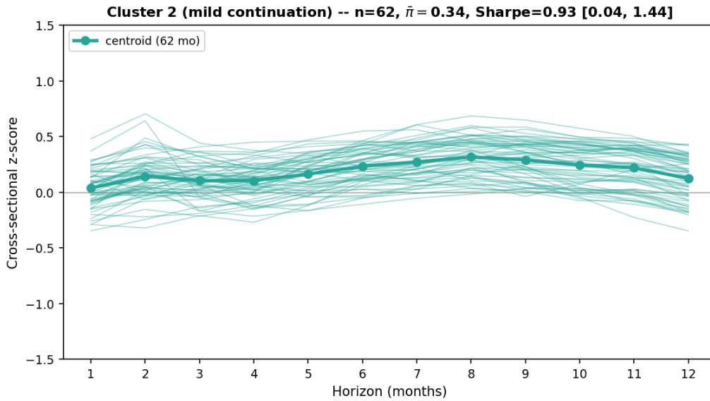
Figure 8: Cluster 2 (mild continuation): z-curves of the 62 member months and centroid. The centroid is mildly positive throughout, peaking at +0.32 at month 8.
