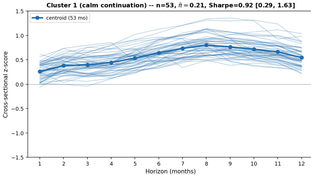
Figure 7: Cluster 1 (calm continuation): z-curves of the 53 member months and centroid. The centroid is humped and uniformly positive, peaking at +0.80 at month 8.
