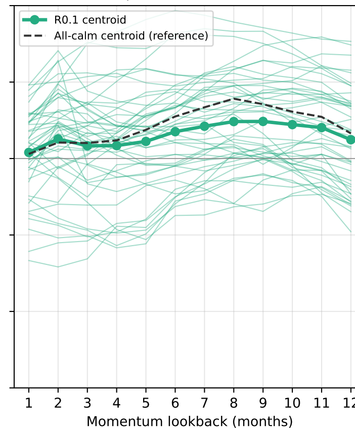
R0.1 — panic-rule \times subshape 1 ( n=45 , \bar{\pi}=0.91 ) Sharpe=1.60 [1.013, 2.445]
