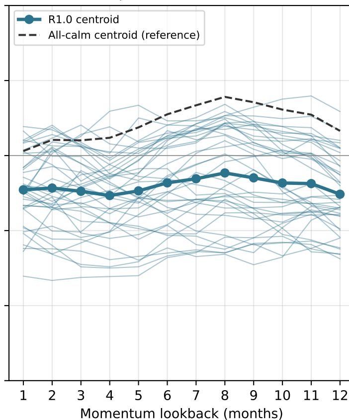
R1.0 — calm-rule \times subshape 0 ( n=38 , \bar{\pi}=0.01 ) Sharpe=0.92 [0.005, 1.789]
