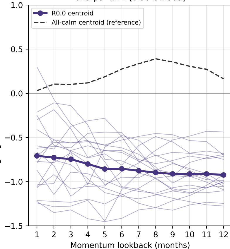
R0.0 — panic-rule \times subshape 0 ( n=18 , \bar{\pi}=1.00 ) Sharpe=1.71 [0.964, 2.563]
