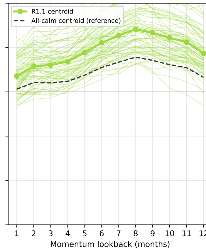
R1.1 — calm-rule \times subshape 1 ( n=66 , \bar{\pi}=0.01 ) Sharpe=0.58 [-0.096, 1.368]
