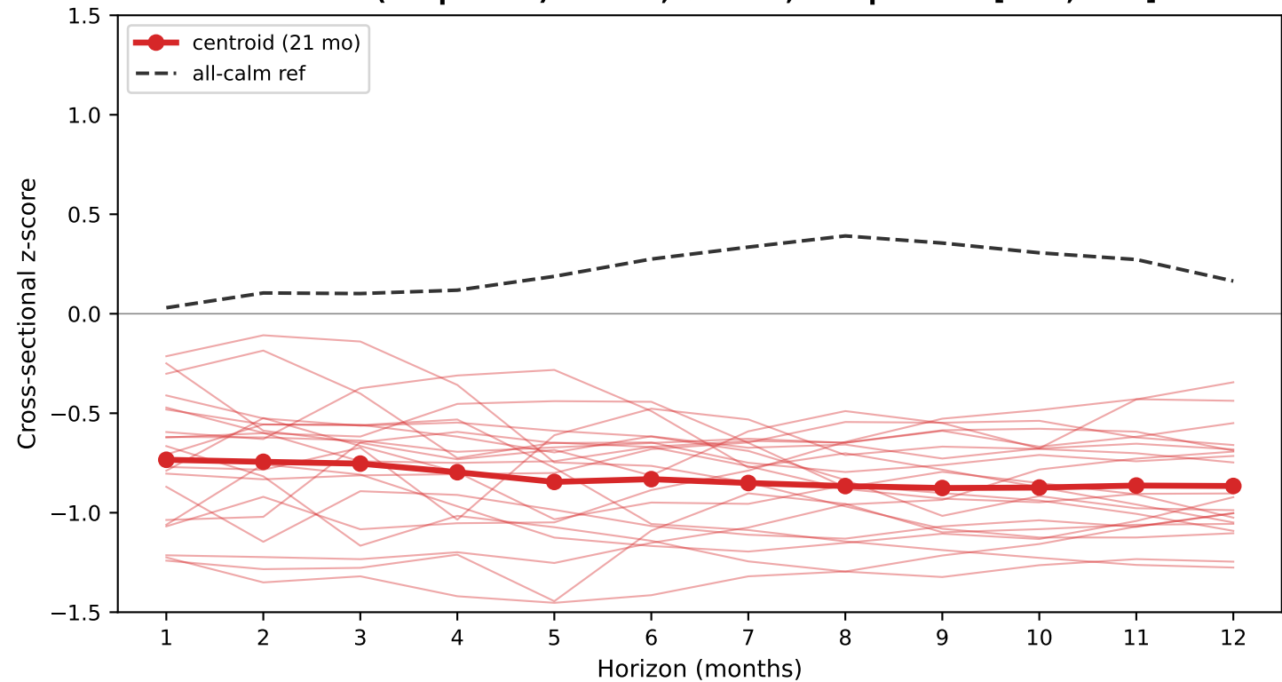
Cluster 4 (deep crisis) -- n=21 , \bar{\pi} = 0.81 , Sharpe=1.82 [0.98, 2.68]
