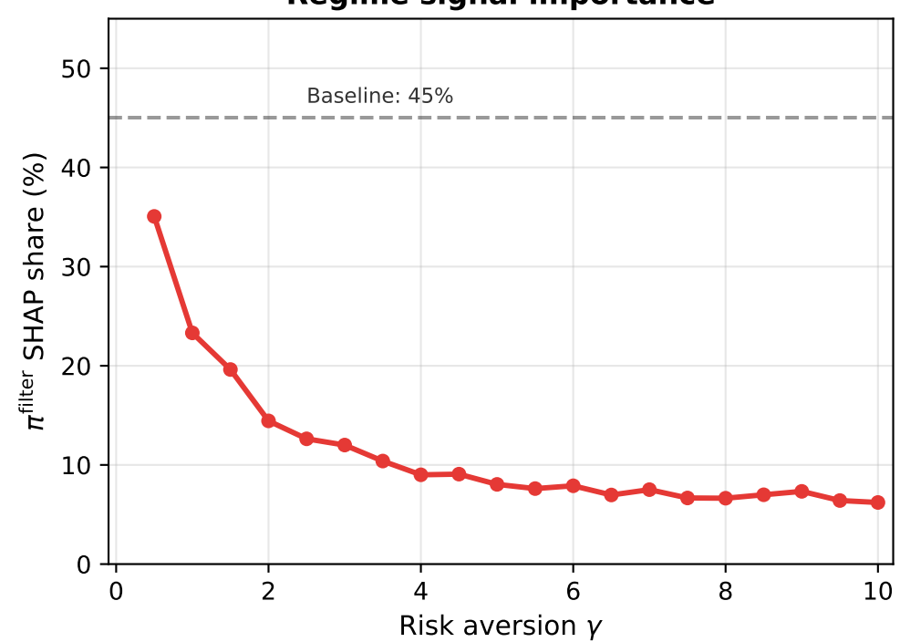
Regime signal importance
