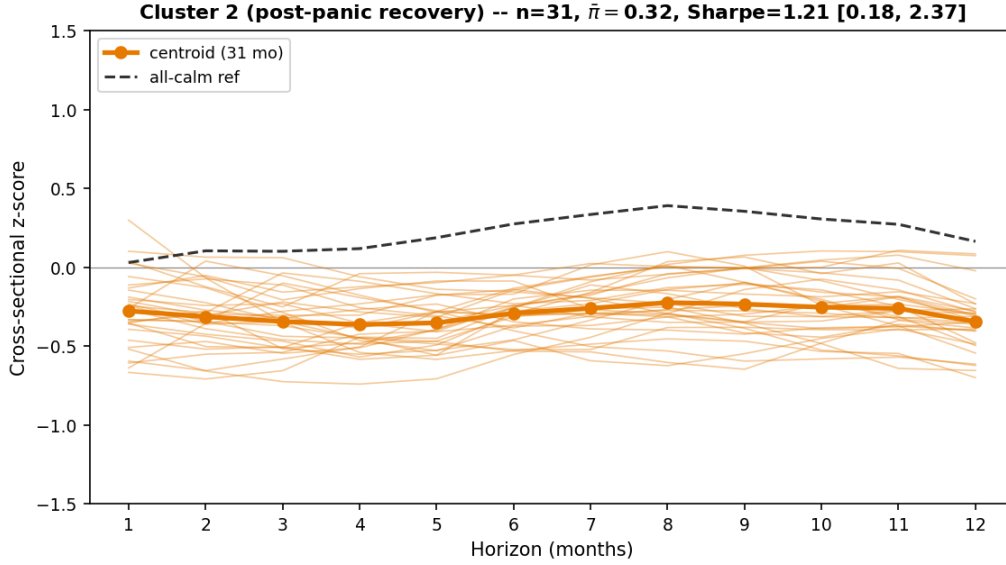
Figure 9: Cluster 2 (post-panic recovery): z-curves of the 31 member months, centroid, and all-calm reference.
