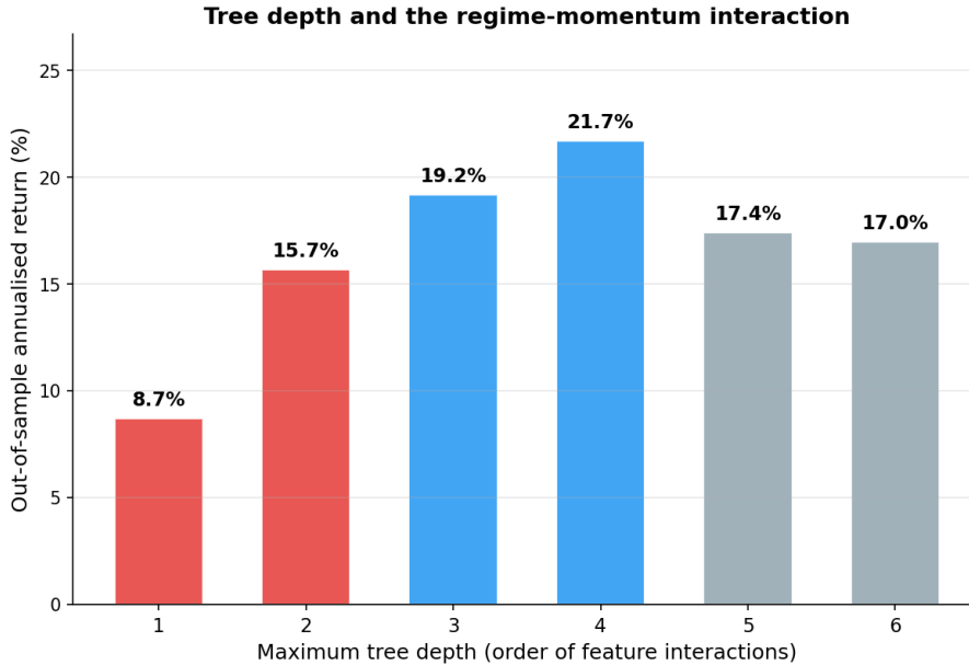
Figure 11: Out-of-sample annualised return as a function of maximum tree depth. Volatility is approximately constant ( \approx 19.5\% ) across all depths.
