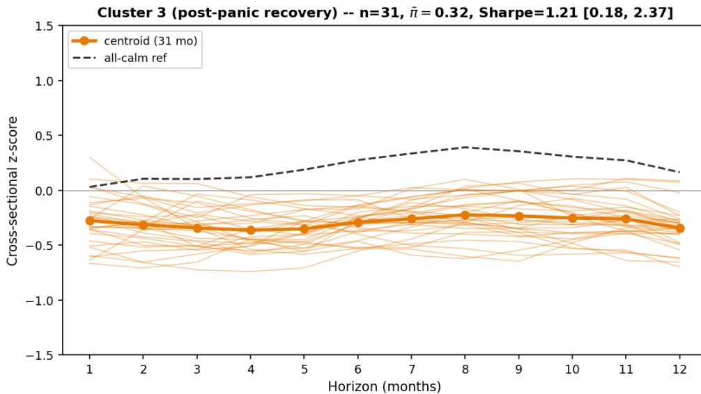
Figure 9: Cluster 3 (post-panic recovery): z-curves of the 31 member months, centroid, and all-calm reference.
