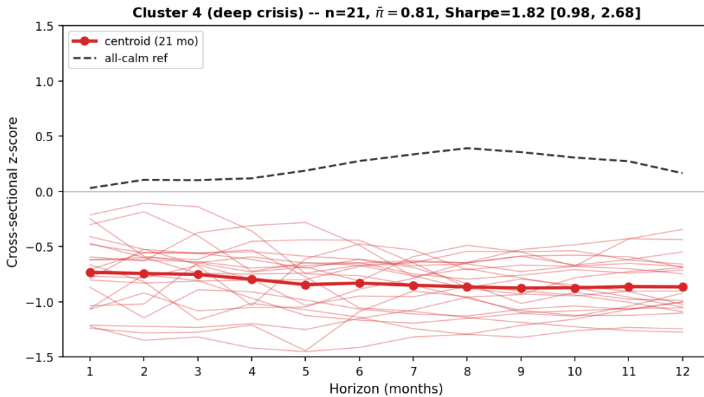
Figure 10: Cluster 4 (deep crisis): z-curves of the 21 member months, centroid, and all-calm reference.
