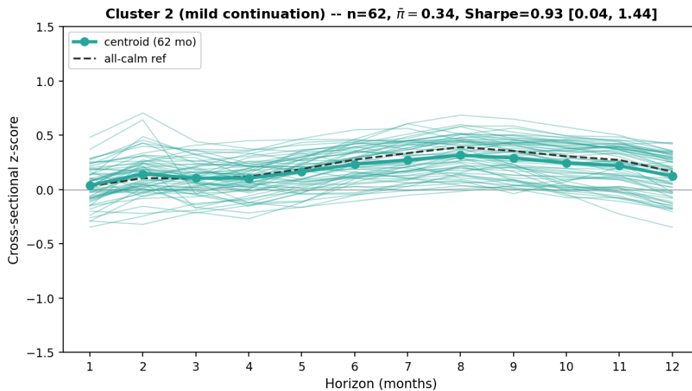
Figure 8: Cluster 2 (mild continuation): z-curves of the 62 member months, centroid, and all-calm reference.
