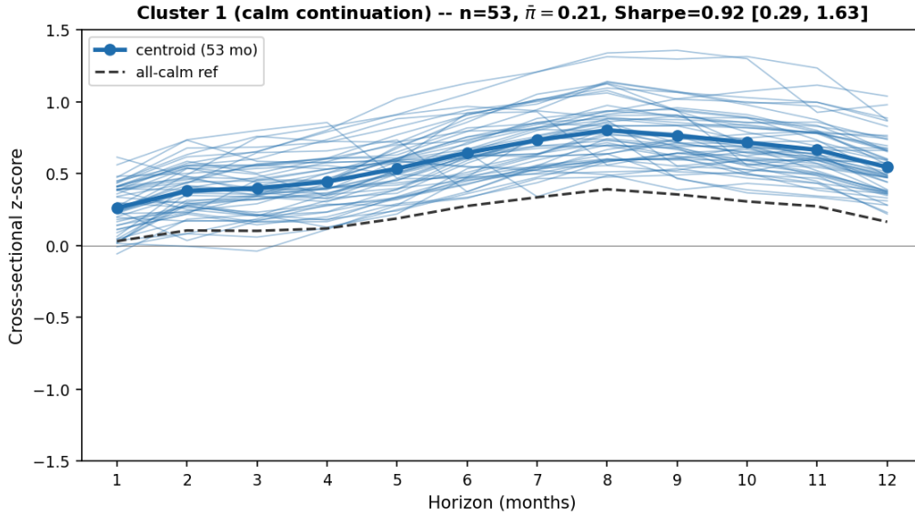
Figure 7: Cluster 1 (calm continuation): z-curves of the 53 member months, centroid, and all-calm reference.
