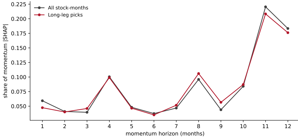
Figure 5: Per-horizon shares of momentum |SHAP| in the main model’s predictions, applied configuration: all out-of-sample stock-months versus the long-leg picks.
