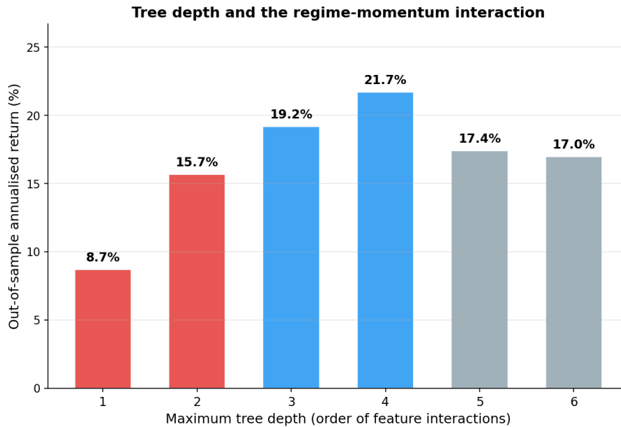
Figure 12: Out-of-sample annualised return as a function of maximum tree depth. Volatility is approximately constant ( \approx 19.5\% ) across all depths.
