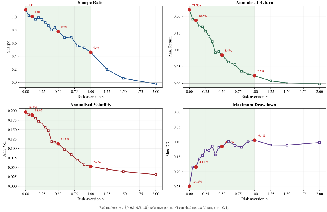
Figure 9: Risk-aversion sweep under the two-model CRRA dual-utility framework. Sharpe ratio, annualised return, annualised volatility, and maximum drawdown as a function of \gamma over [0, 2] . Red markers highlight \gamma \in \{0, 0.1, 0.5, 1.0\} ; green shading indicates the useful range \gamma \in [0, 1] .
