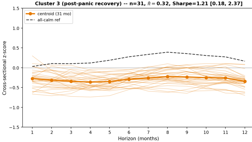
Figure 9: Cluster 3 (post-panic recovery): z-curves of the 31 member months, centroid, and all-calm reference.
