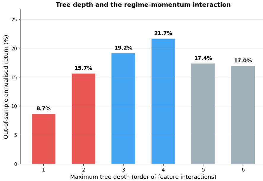
Figure 11: Out-of-sample annualised return as a function of maximum tree depth. Volatility is approximately constant ( \approx 19.5\% ) across all depths.
