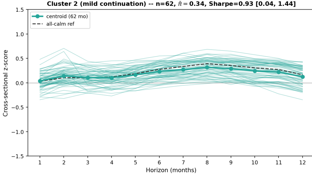
Figure 8: Cluster 2 (mild continuation): z-curves of the 62 member months, centroid, and all-calm reference.
