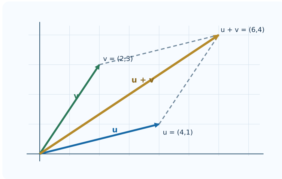
Figura 3.2: La diagonal representa u + v .
