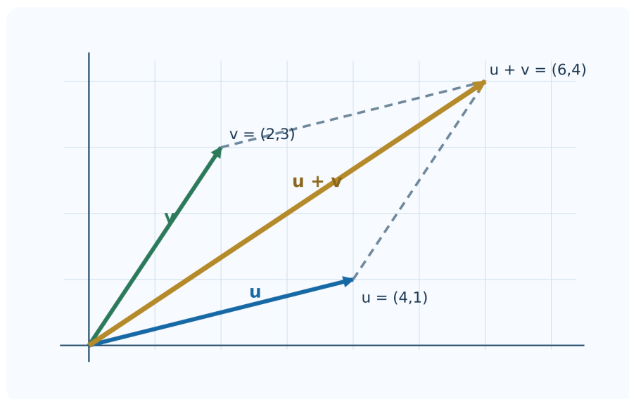
Figura 3.2: La diagonal representa u + v .
