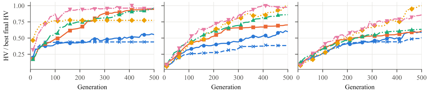
A-n32-k5 (3 seeds)
