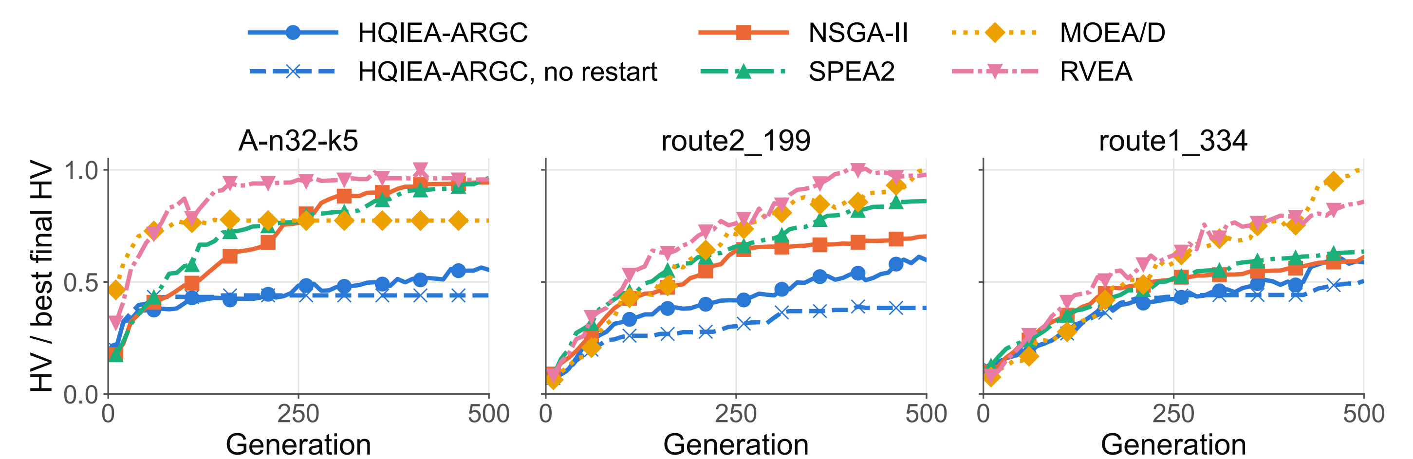
Figure 1: HV per generation, normalised to the best final HV (median of 3 seeds). Without restart (dashed) HQIEA-ARGC stalls (A-n32-k5: from about generation 60) while most baselines keep climbing.
