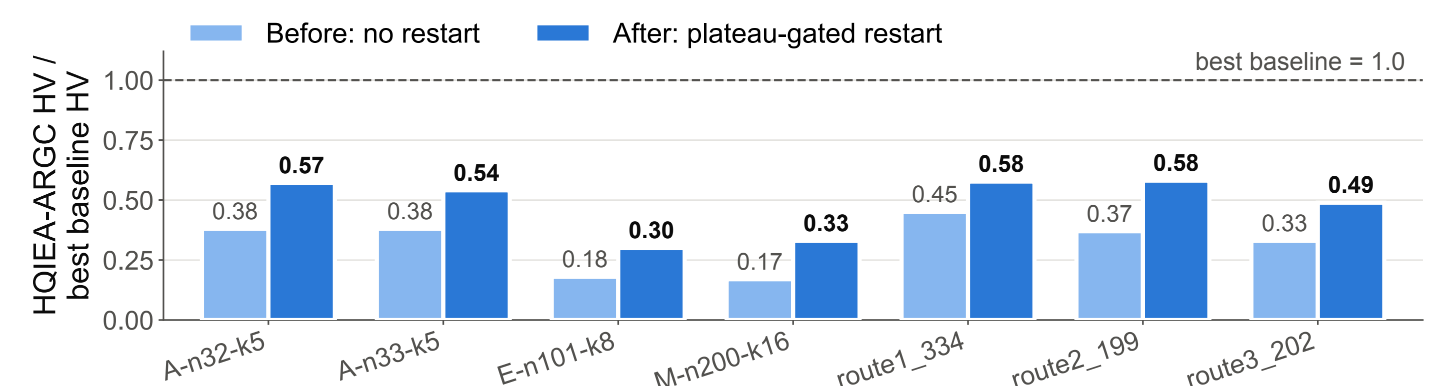
Figure 2: Mean HV relative to the best baseline (30 runs \times 500 generations).
