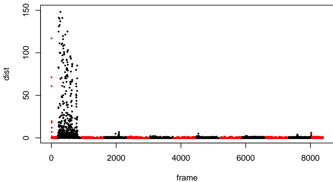
20140425-175349_0: ID: 4; sp: H_a
