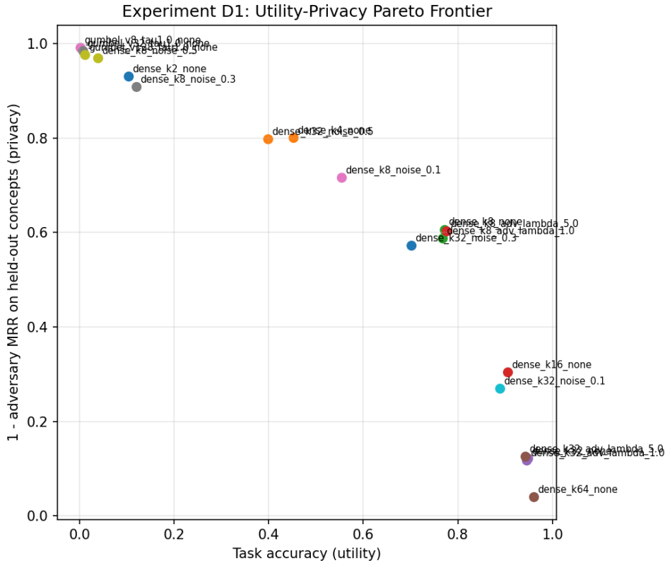
Figure 28: Experiment D1. Utility (task accuracy) vs privacy (1–adversary MRR on held-out concepts). The clean dense bottleneck sweep ( k = 2 to 64 , blue through brown) traces a smooth monotonic frontier from high-privacy/low-utility to low-privacy/high-utility. Noise defenses (orange/grey/cyan/pink) sit close to this same frontier rather than displacing it. Adversarial training (green/red/purple/brown clusters near k = 8 and k = 32 ) produces negligible movement relative to the corresponding undefended k . Gumbel configurations (top left) achieve near-perfect privacy but at essentially zero task accuracy.
