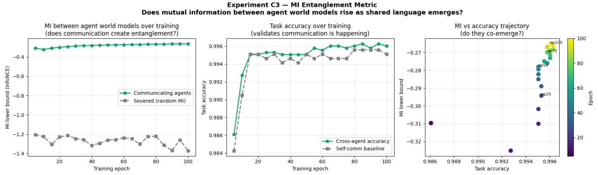
Figure 27: Experiment C3. Left : MI lower bound over training — communicating agents (green) rise; severed baseline (grey) flat. Centre : task accuracy. Right : MI vs accuracy trajectory.
