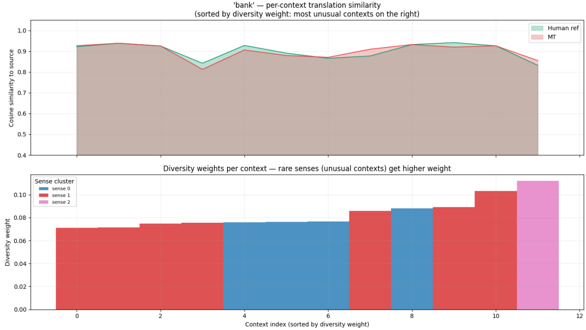
Figure 11: Per-context translation similarity for bank (sorted by diversity weight, most unusual contexts on the right). Top : human reference and MT similarity traces — nearly overlapping, with human reference slightly higher on average. Bottom : diversity weights by sense cluster. The single Sense 2 context (pink, far right) receives the highest diversity weight (0.115); because MT outperforms the human reference on that context, the weighted gap is smaller than the unweighted gap.
