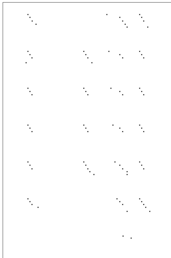
Drill Map: • 0.200mm / 0.0079" (82 holes)
